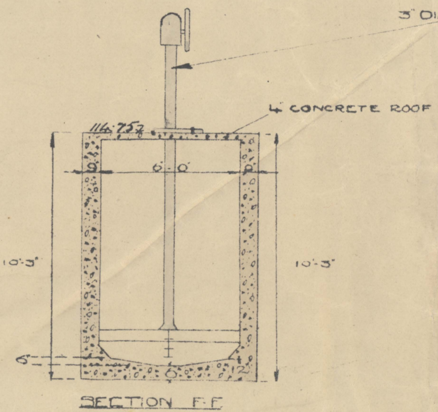
SECTION F-F
