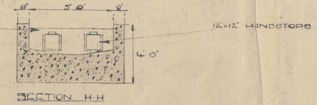
SECTION H-H
