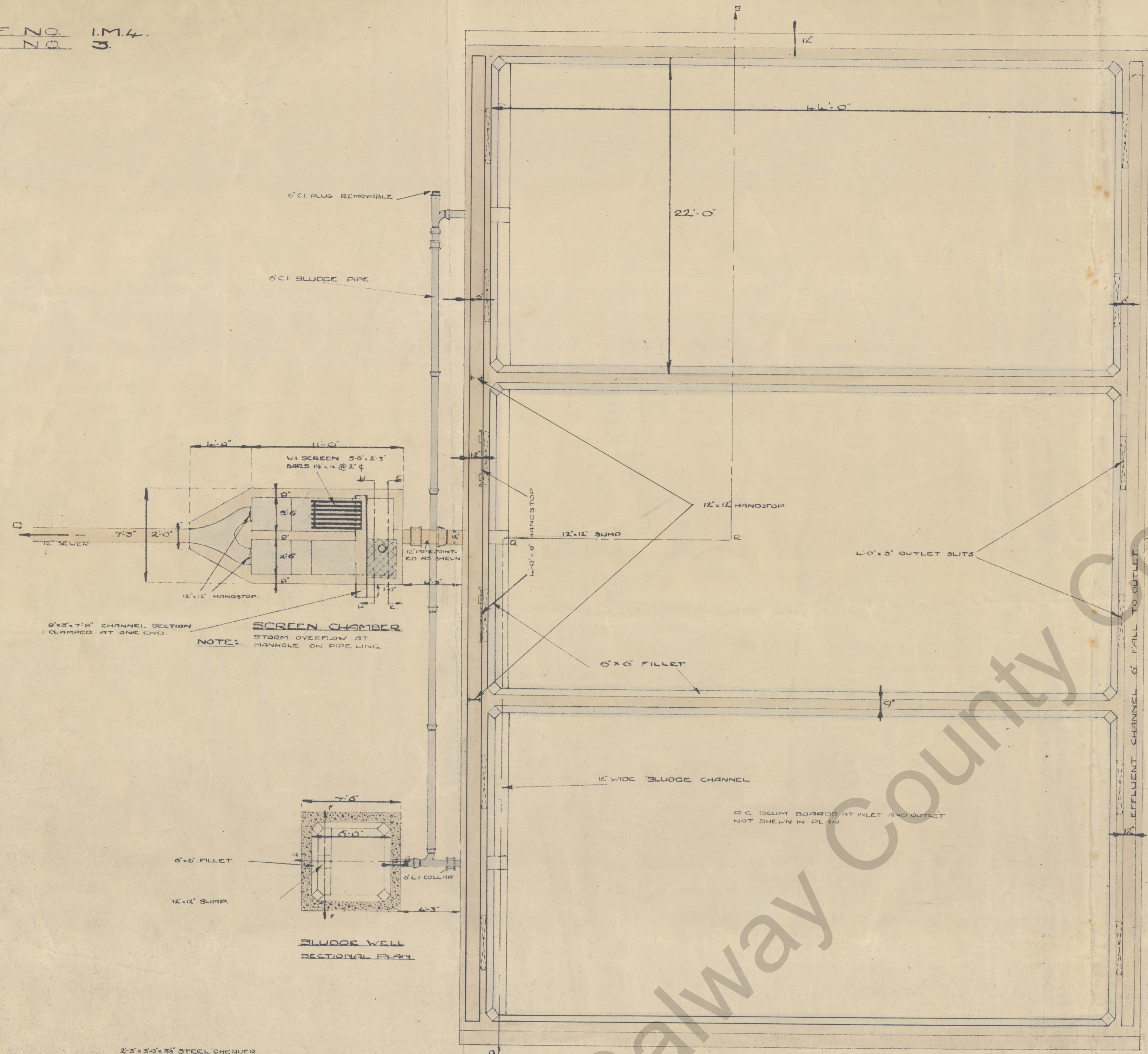
LAYOUT PLAN
