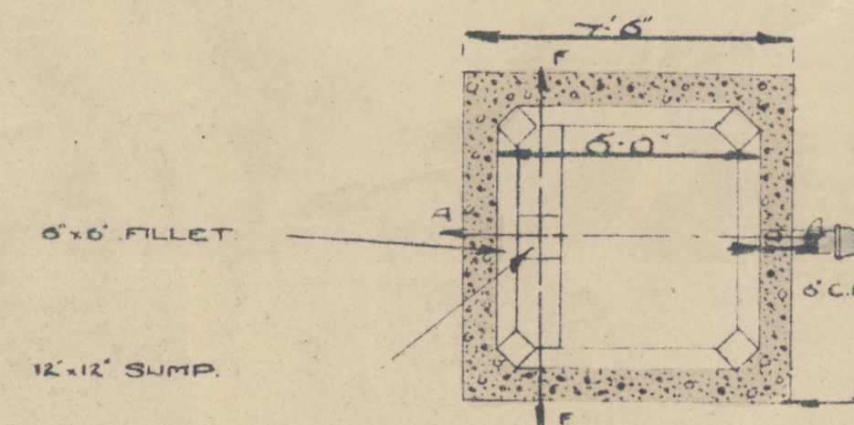
SLUDGE WELL
